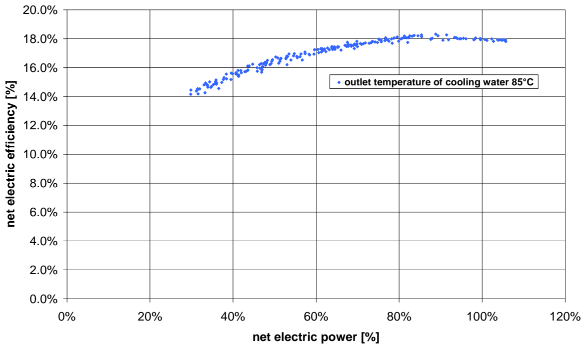
Figure 7: Net electric efficiency vs. load of the ORC unit according to measured data – biomass CHP plant in Lienz
